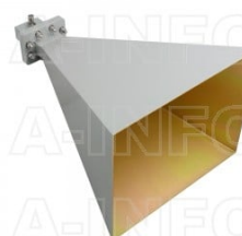
LB-187-20-C-TF Standard Gain Horn Antenna 3.95-5.85GHz 20dB Gain TNC Female
